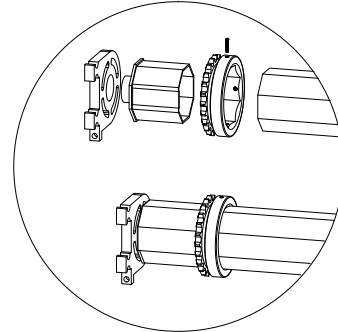
DETAIL "E"
